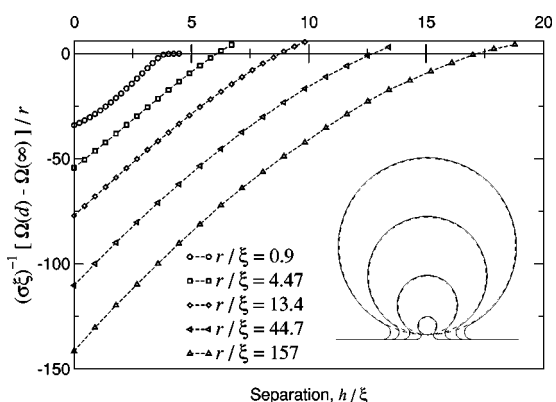
FIG. 8. Excess free energy of the configuration with the bridge vs sphere-plane separation. Different curves correspond to different sphere radii. Inset illustrates change in the radial extent and shape of the bridge when the sphere radius changes. The inset configurations are taken at a fixed sphere-surface separation, h/\xi = 8.94 .
